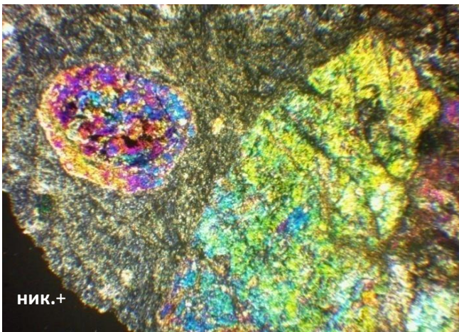
Copper ore. Pseudomorph chlorite-epidote in cryptocrystalline matrix of the rock. Polished section. Nicol +, x100
